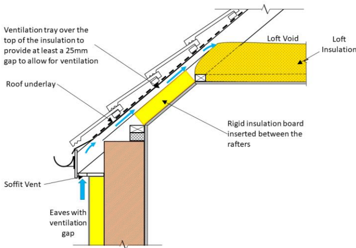
Figure 20 Skelling Insulated with Rigid Insulation Board Between the Rafters
