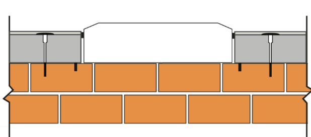
Figure 3 EWI Installed around and sealed against the meter box
