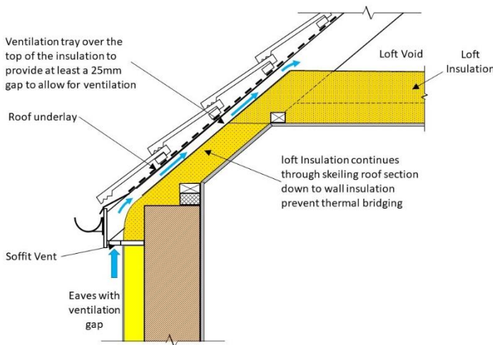
Figure 18 Skelling Insulated with Loft Insulation Between the Rafters
