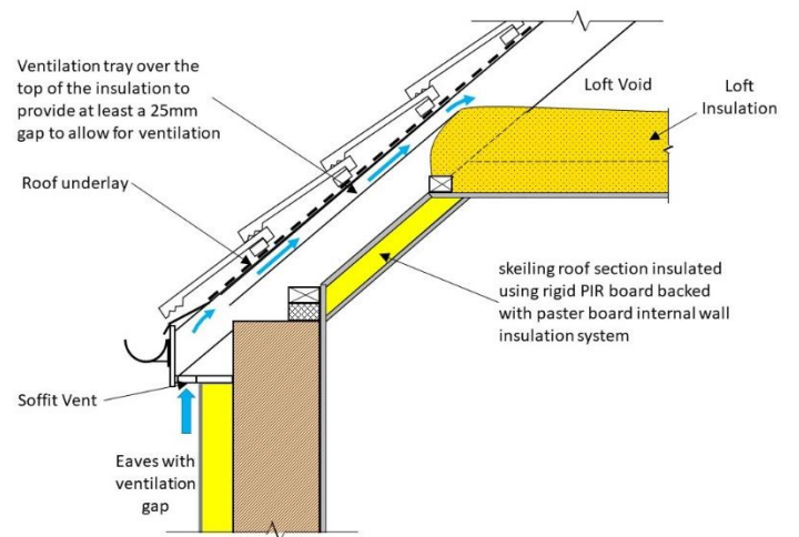
Figure 19 Skelling Insulated with Internal Wall Insulation
